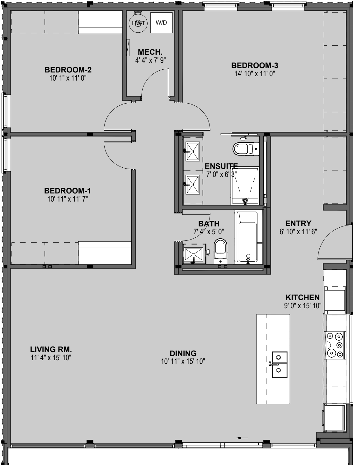
HO4 TYPE-2 KITCHEN RIGHT TOTAL SIZE: 32'X42' (1,344 SF) UNIT SIZE: 32' X 40' (1,280 SF) (STANDARD)
