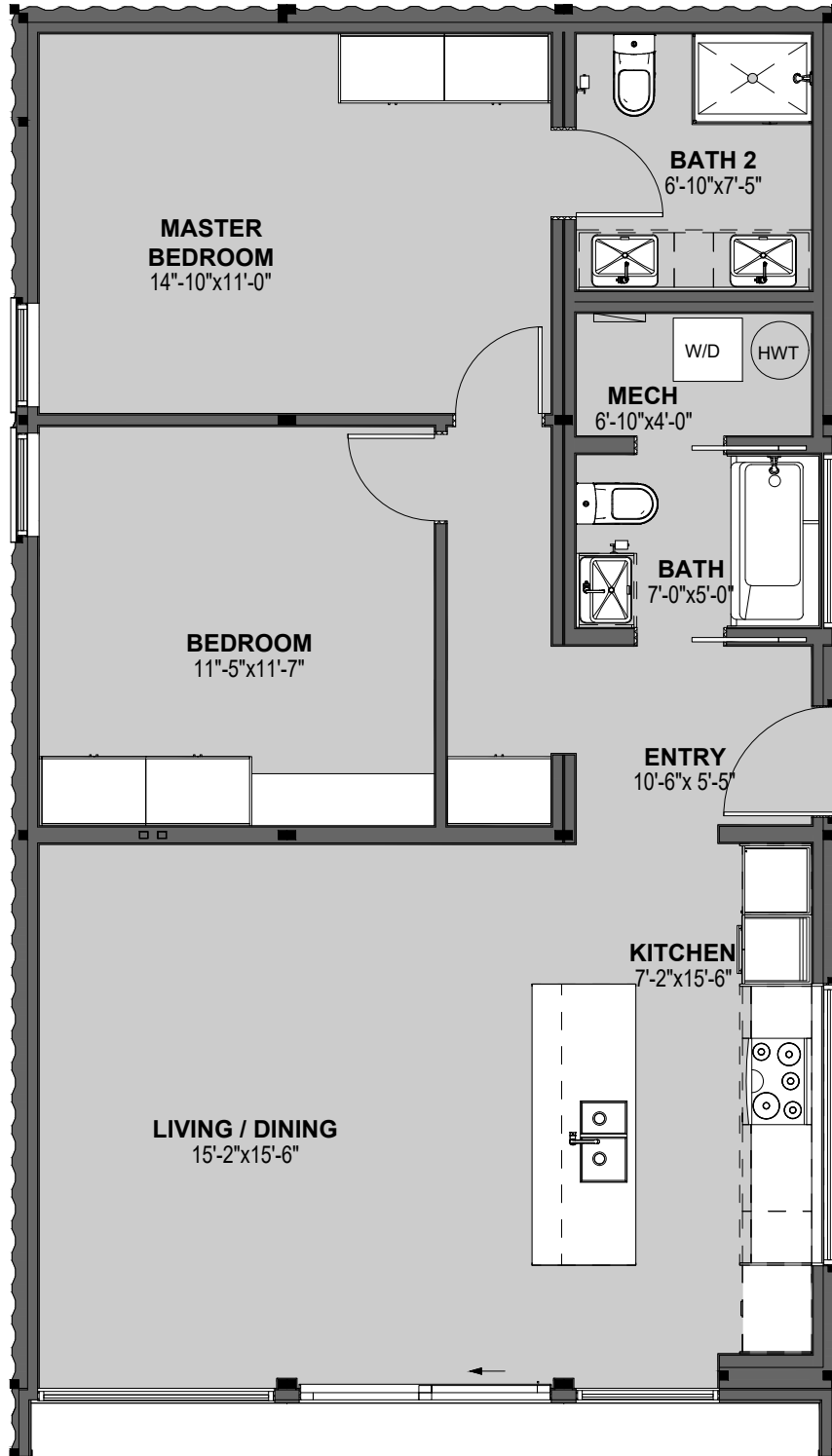
HO3 TYPE-2 KITCHEN RIGHT TOTAL SIZE: 24' X 42' (1,008 SF) UNIT SIZE: 24' X 40' (960 SF) (STANDARD)
